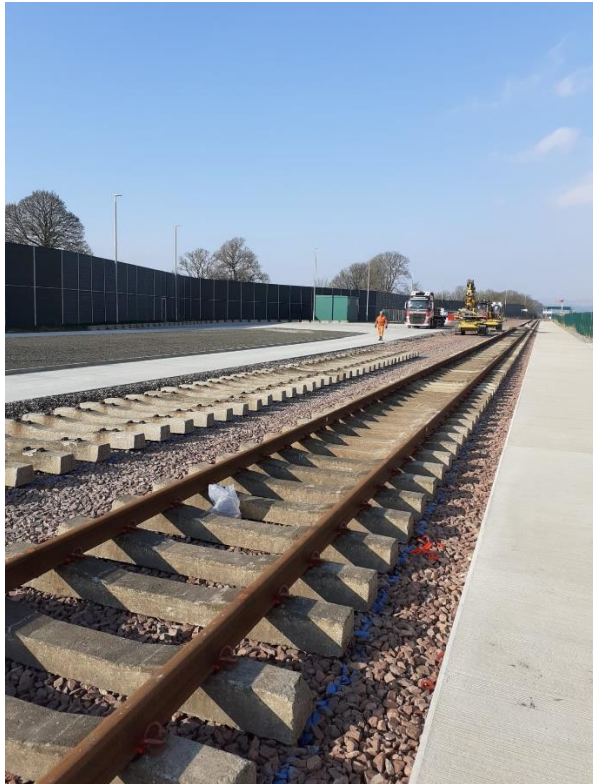
Figures 12-14 – Installation of sleepers and rails for sidings No. 1 & No. 2
