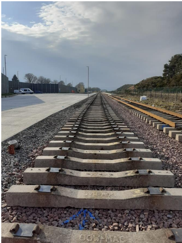
Figures 12-14 – Installation of sleepers and rails for sidings No. 1 & No. 2
