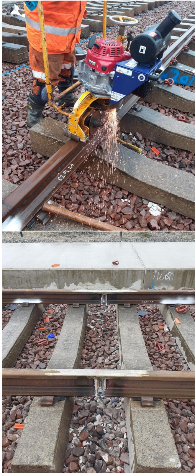
Figures 15-16 – Track Welding
